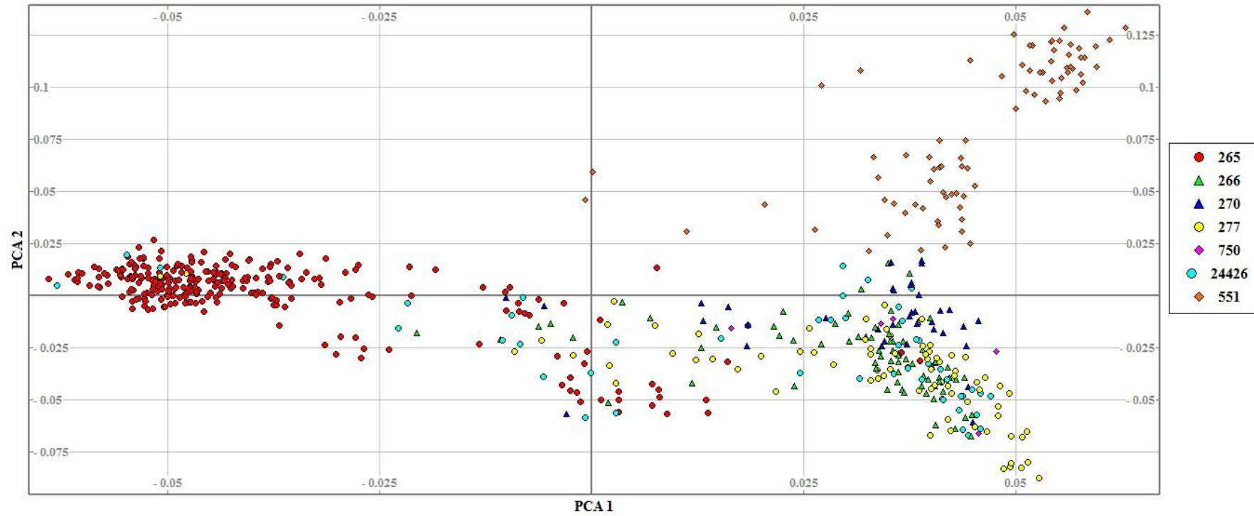
Figure 4 SNP-based Principal Component Analysis (PCA) of 588 Gyr cattle from 7 subpopulations.
